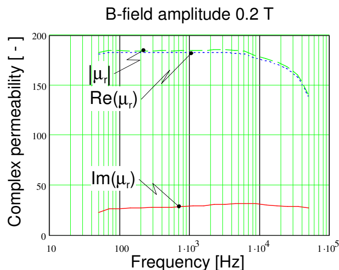
Figure 4. The complex, relative permeability as a function of the frequency ranging from 50 - 50000 Hz, measured at constant amplitude, 0.2 T, of the magnetic flux density.
