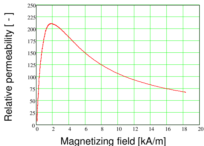
Figure 2. The relative permeability deduced from the virginal magnetization loop in Figure 1.
